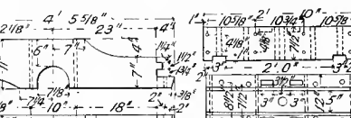
Figs. 5074-75. 5076-77. 5078-79 5080-81. BRAKE-HANGER AND U-BOLT.
